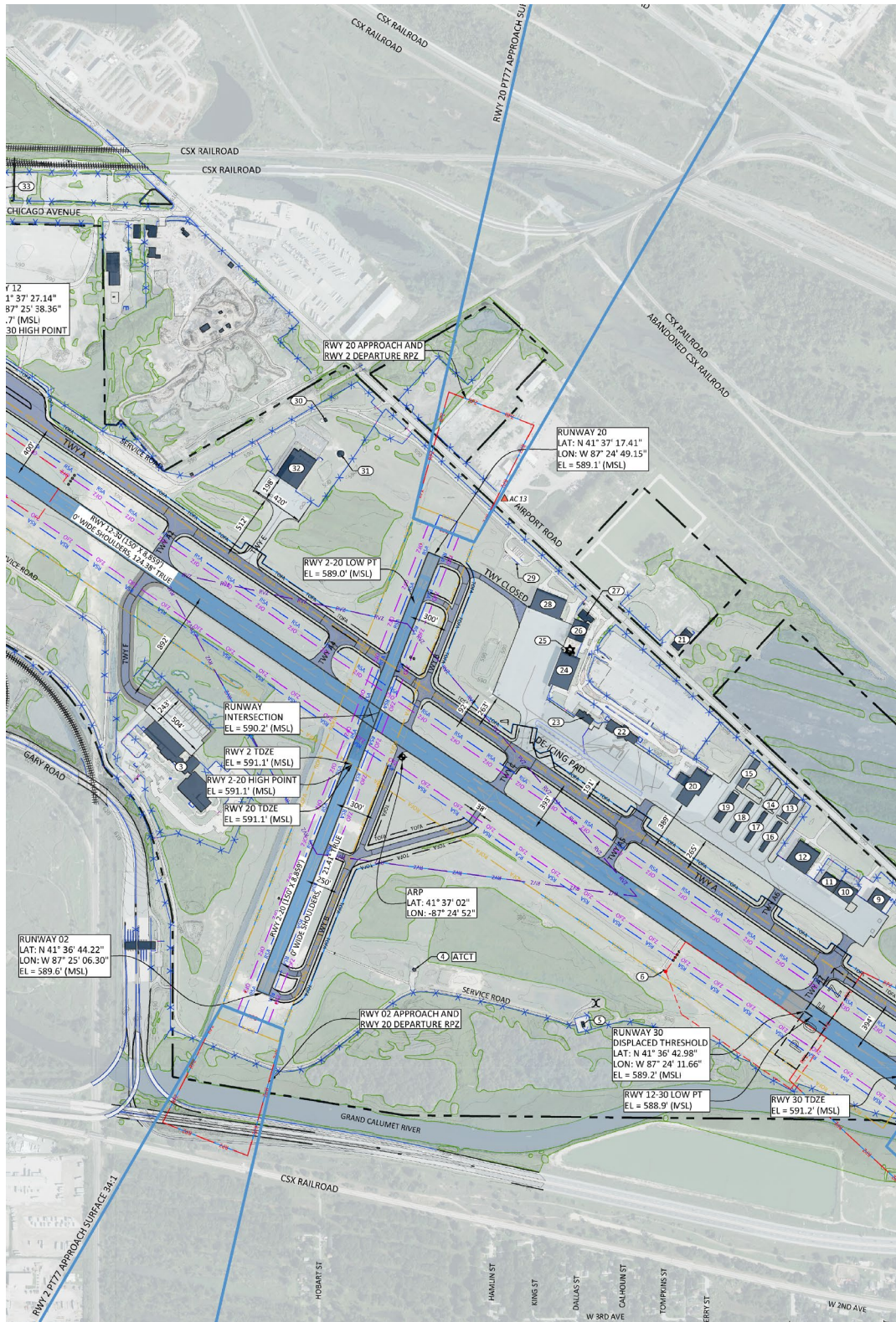
Figure 3-2 – Runway 2-20 Exiting Geometry and Environs
