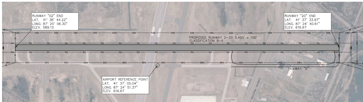
Figure 3-3 – Existing Runway 2-20 Extension Plan on File
